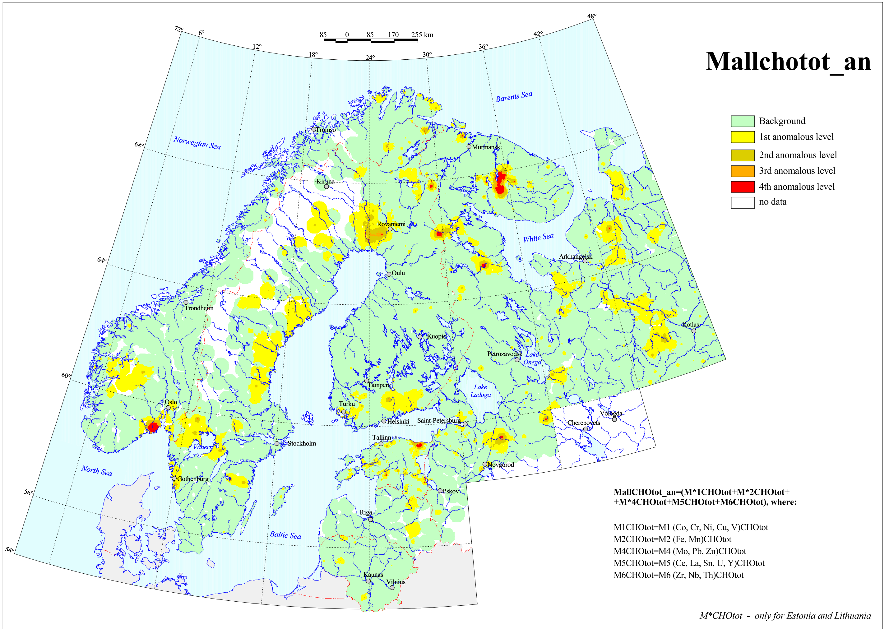
Integrated Anomalous Geochemical Fields, Mallchotot_an
